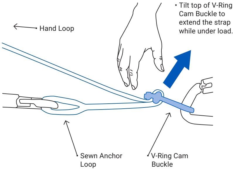
A PROPERLY THREADED V-RING CAM BUCKLE
